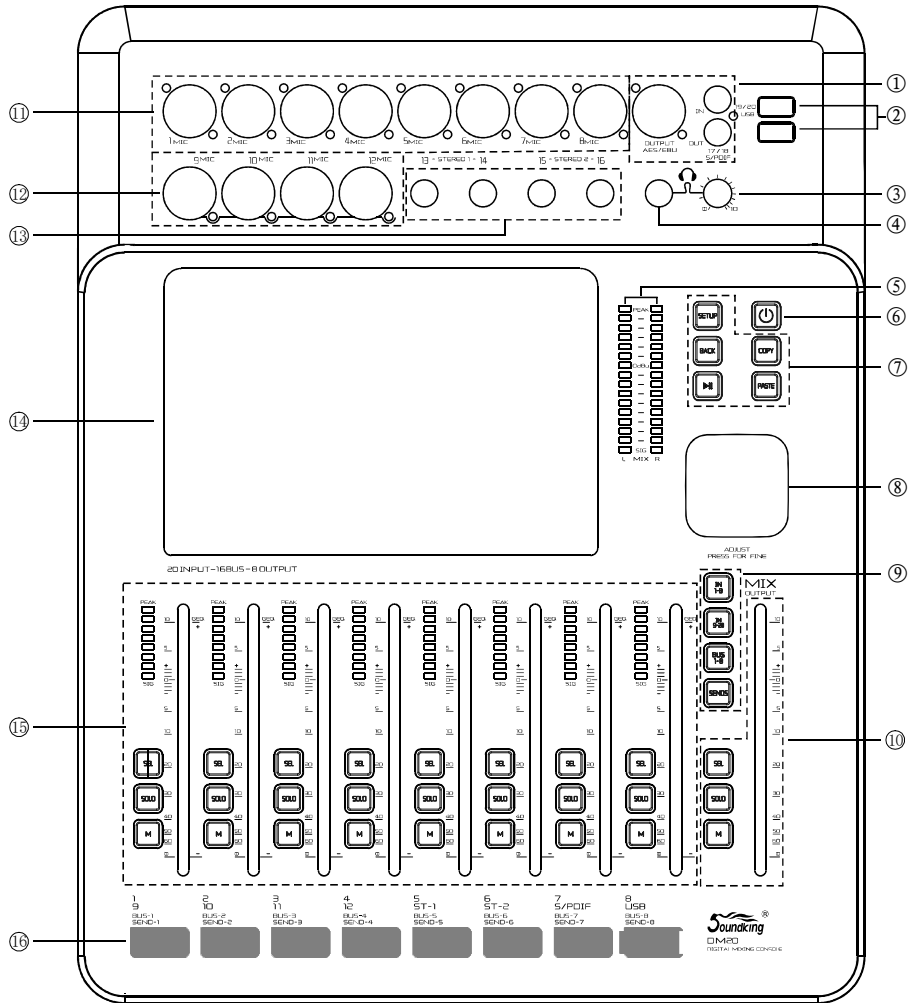
(DM20 Mixer panel)
